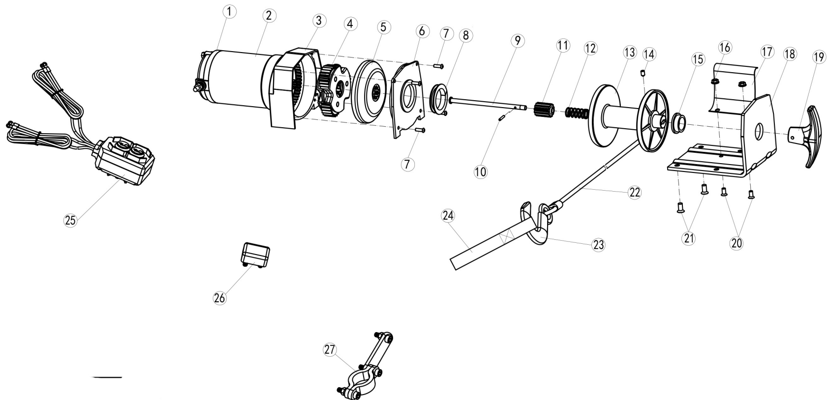
KM2000-1 part list
